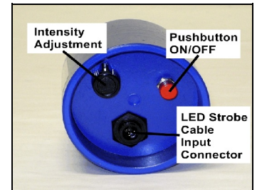
LED Strobe Light Back with callouts.
